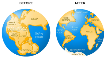
CONTINENTAL DRIFT
